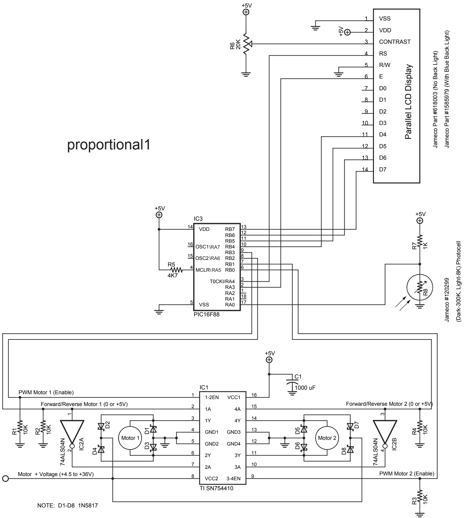
Texas Instrument SN754410 H-Bridge Motor Driver
